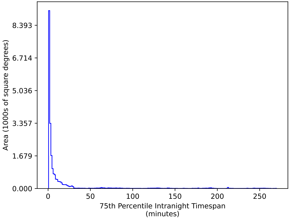
weather_cloudso18v3.4_10yrs All sky u band: 75th Percentile Intranight Timespan
