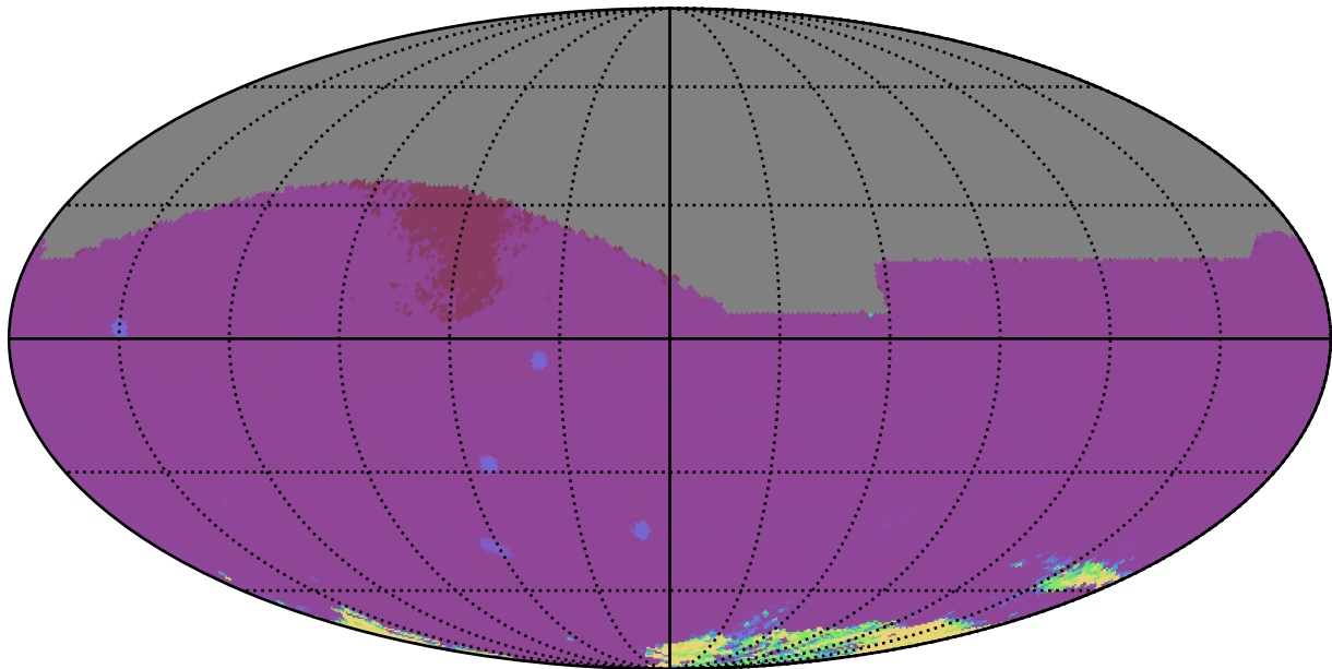
weather_cloudso18v3.4_10yrs All sky iz bands: 75th Percentile Intranight Timespan
