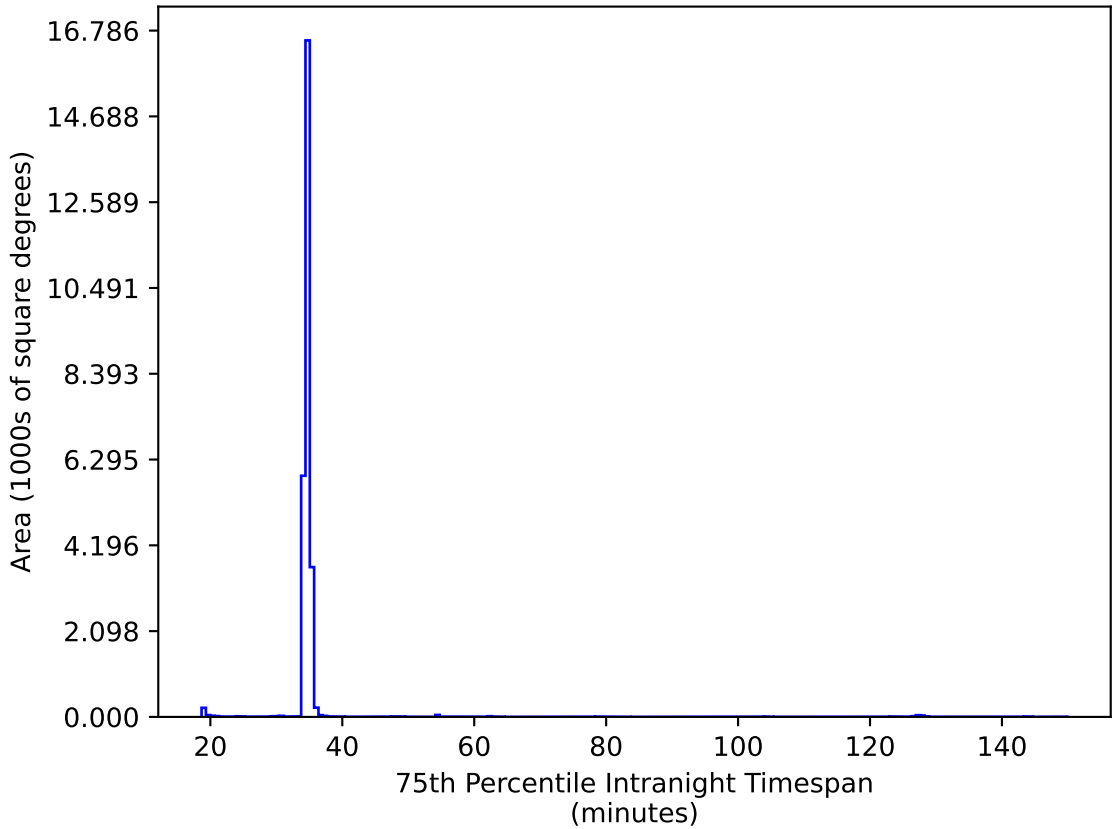
weather_cloudso18v3.4_10yrs All sky iz bands: 75th Percentile Intranight Timespan
