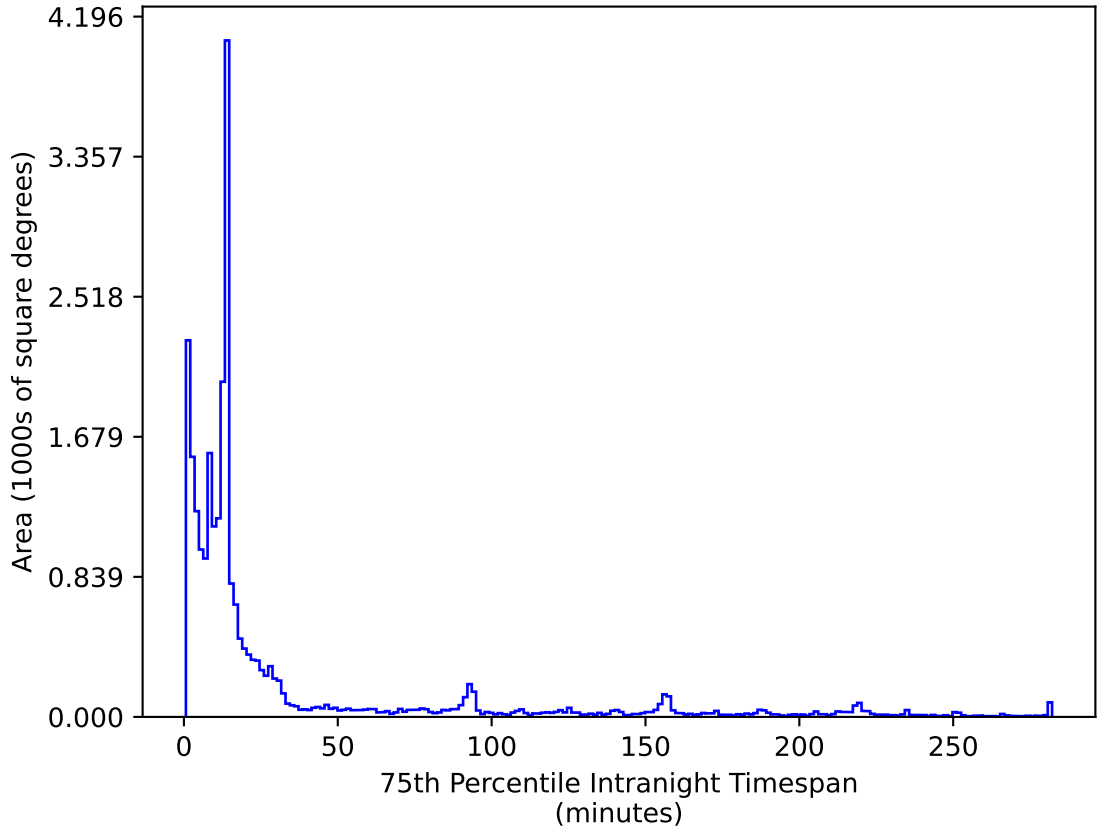
weather_cloudso18v3.4_10yrs All sky i band: 75th Percentile Intranight Timespan
