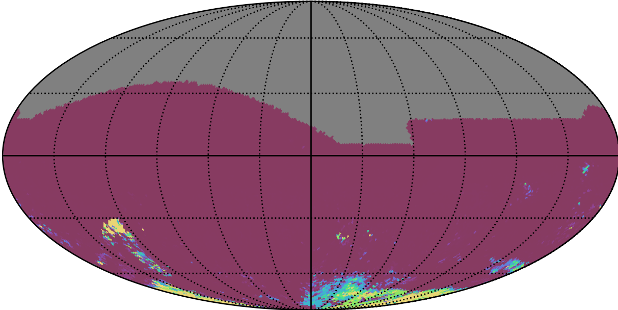
weather_cloudso18v3.4_10yrs All sky gr bands: 75th Percentile Intranight Timespan
