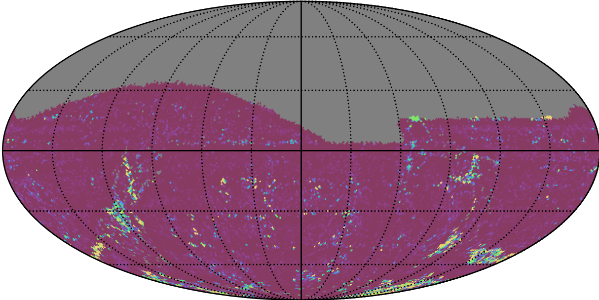
weather_cloudso18v3.4_10yrs All sky g band: 75th Percentile Intranight Timespan
