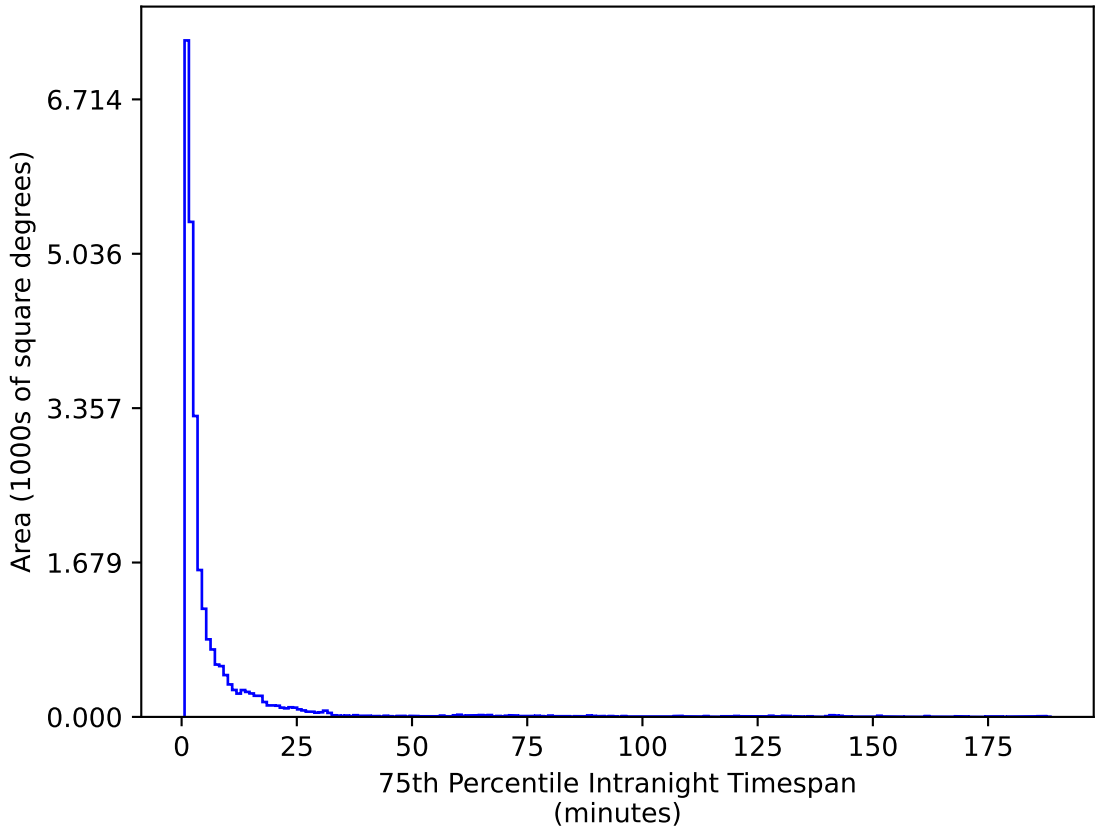
weather_cloudso18v3.4_10yrs All sky g band: 75th Percentile Intranight Timespan
