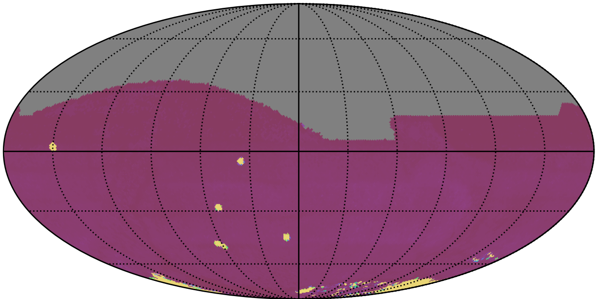
weather_cloudso18v3.4_10yrs All sky all bands: 75th Percentile Intranight Timespan
