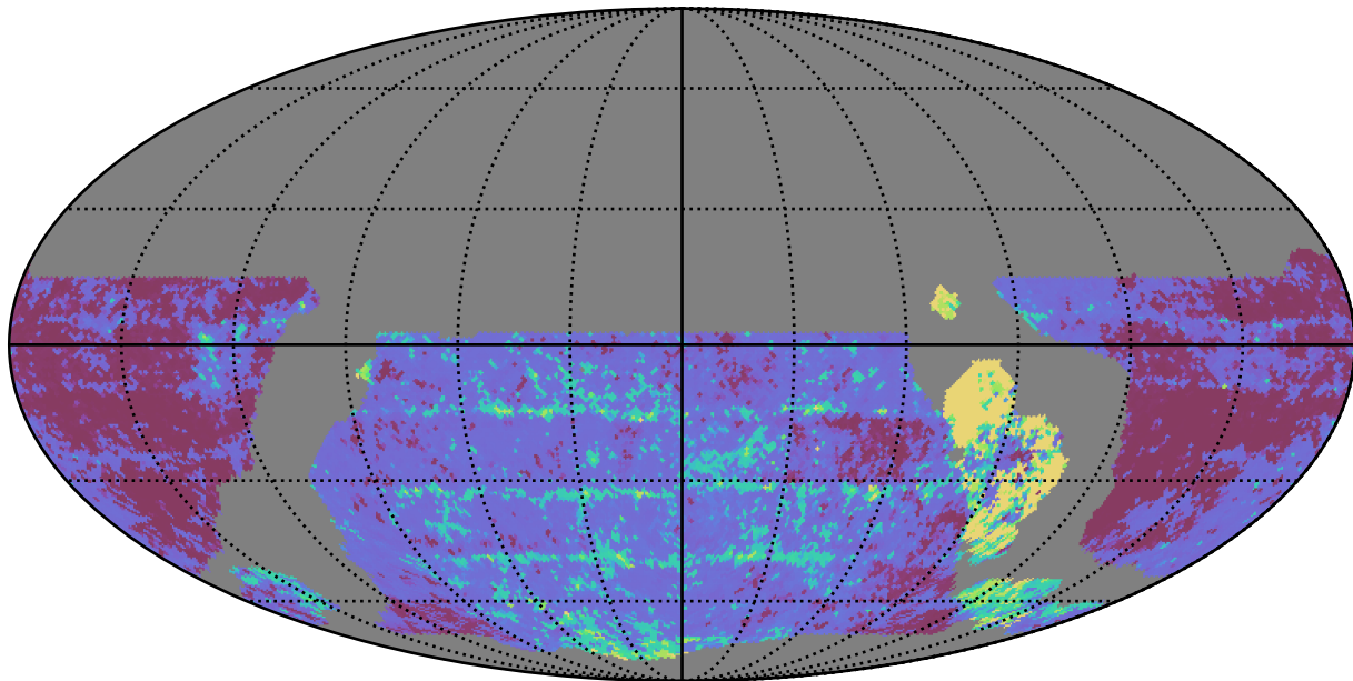
weather_cloudso18v3.4_10yrs WFD y band: 20thPercentile Inter-Night Gap
