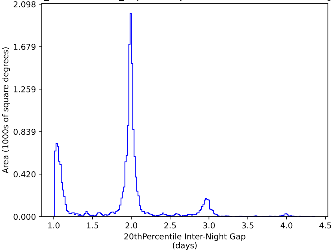
weather_cloudso18v3.4_10yrs WFD y band: 20thPercentile Inter-Night Gap
