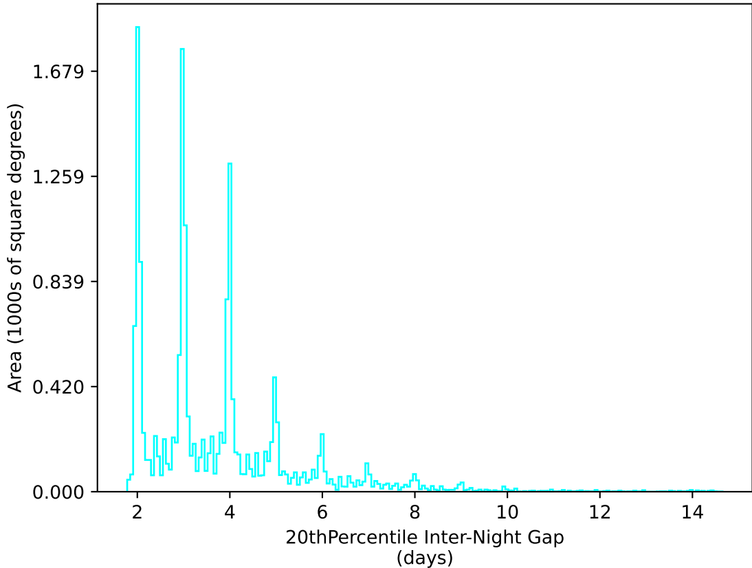
weather_cloudso18v3.4_10yrs WFD u band: 20thPercentile Inter-Night Gap
