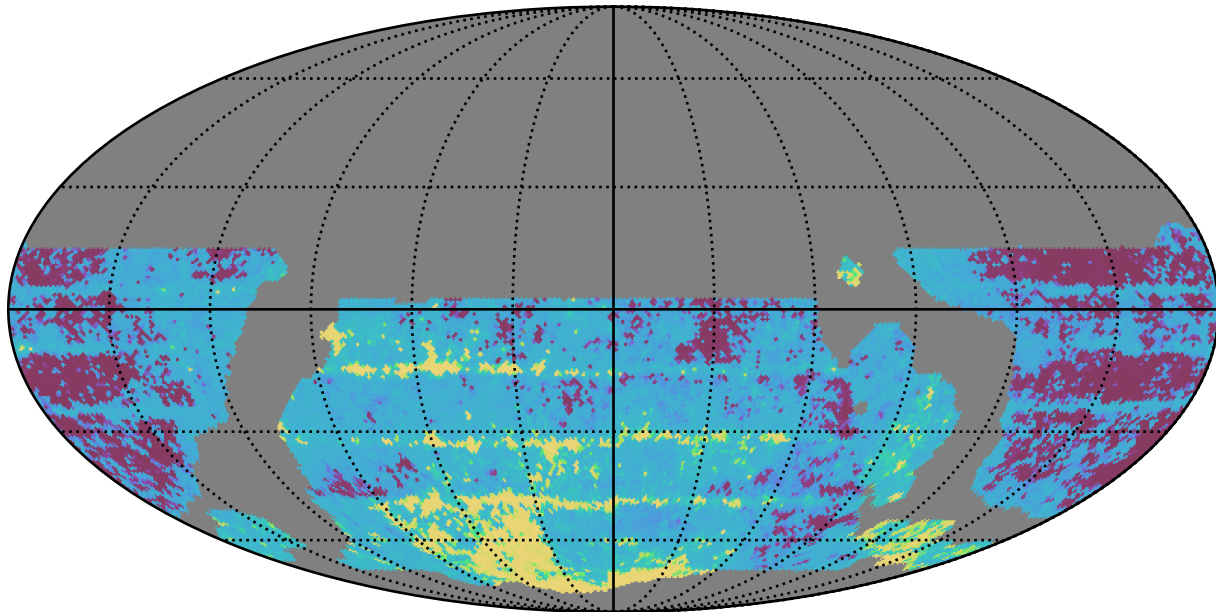
weather_cloudso18v3.4_10yrs WFD r band: 20thPercentile Inter-Night Gap
