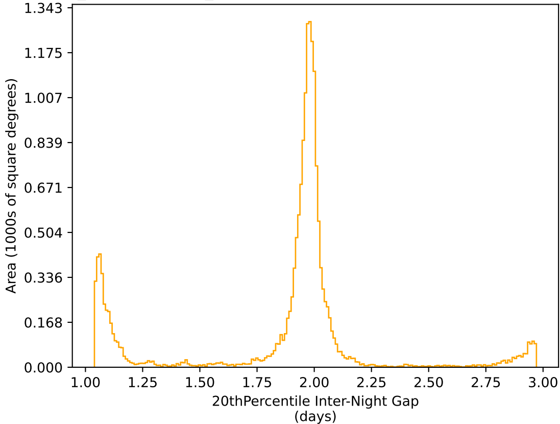
weather_cloudso18v3.4_10yrs WFD r band: 20thPercentile Inter-Night Gap
