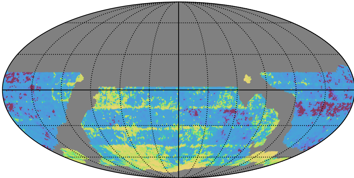
weather_cloudso18v3.4_10yrs WFD i band: 20thPercentile Inter-Night Gap
