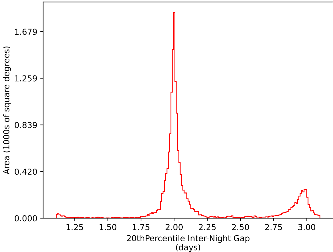
weather_cloudso18v3.4_10yrs WFD i band: 20thPercentile Inter-Night Gap
