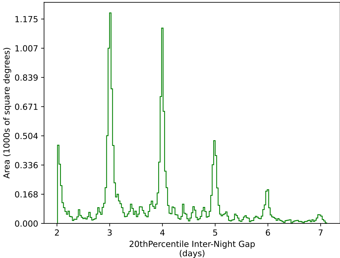
weather_cloudso18v3.4_10yrs WFD g band: 20thPercentile Inter-Night Gap
