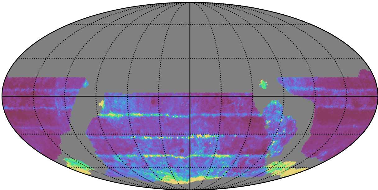
weather_cloudso18v3.4_10yrs WFD all bands: 20thPercentile Inter-Night Gap
