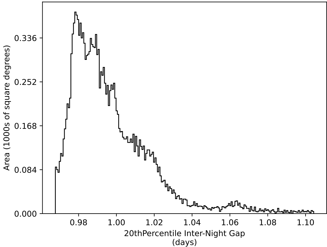
weather_cloudso18v3.4_10yrs WFD all bands: 20thPercentile Inter-Night Gap
