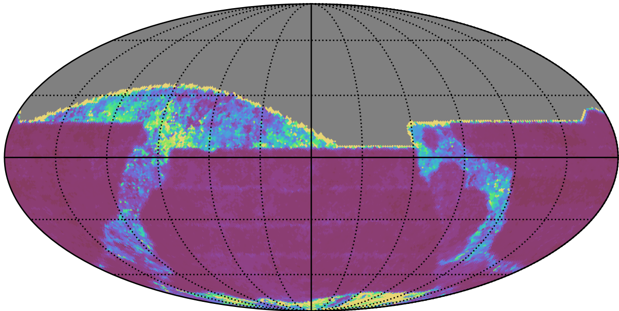
weather_cloudso18v3.4_10yrs All sky z band: 20thPercentile Inter-Night Gap
