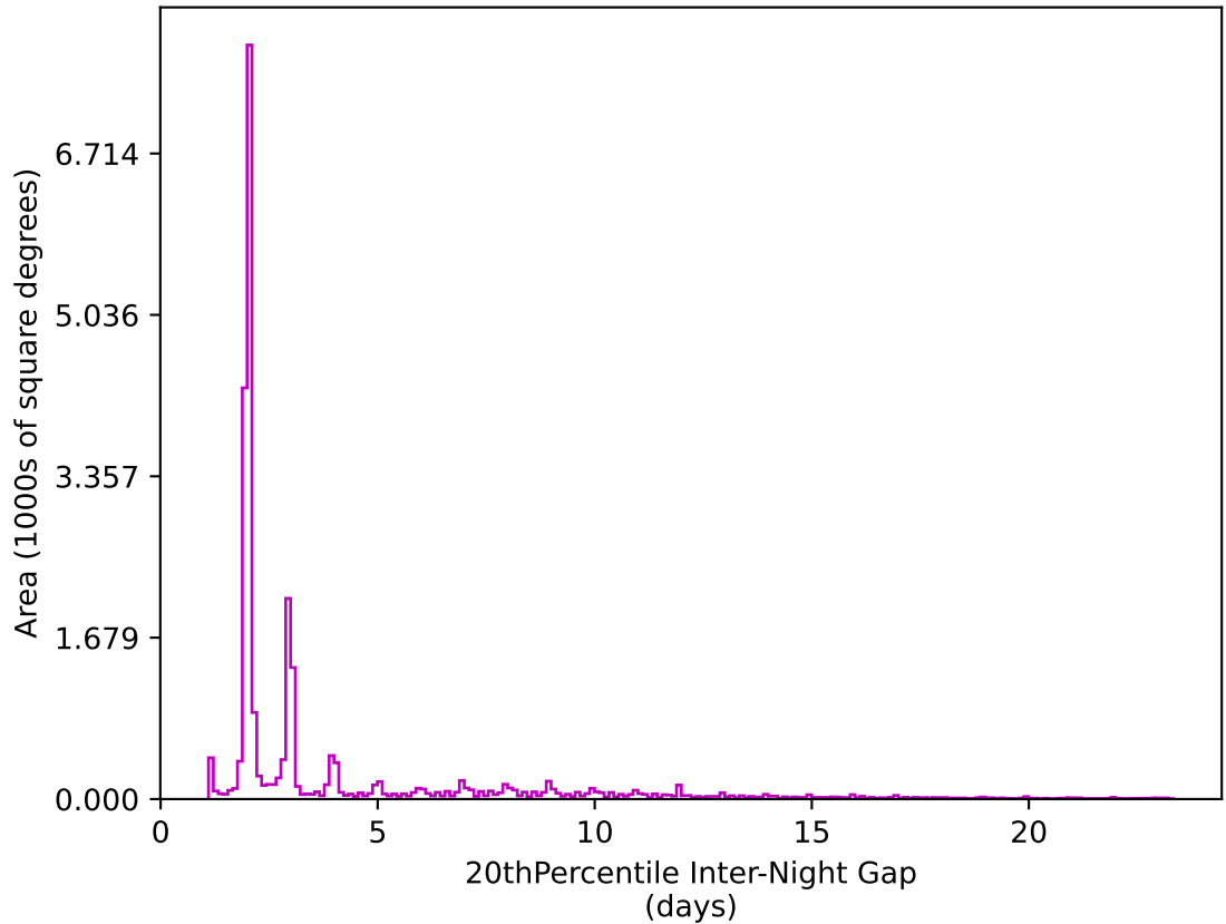
weather_cloudso18v3.4_10yrs All sky z band: 20thPercentile Inter-Night Gap
