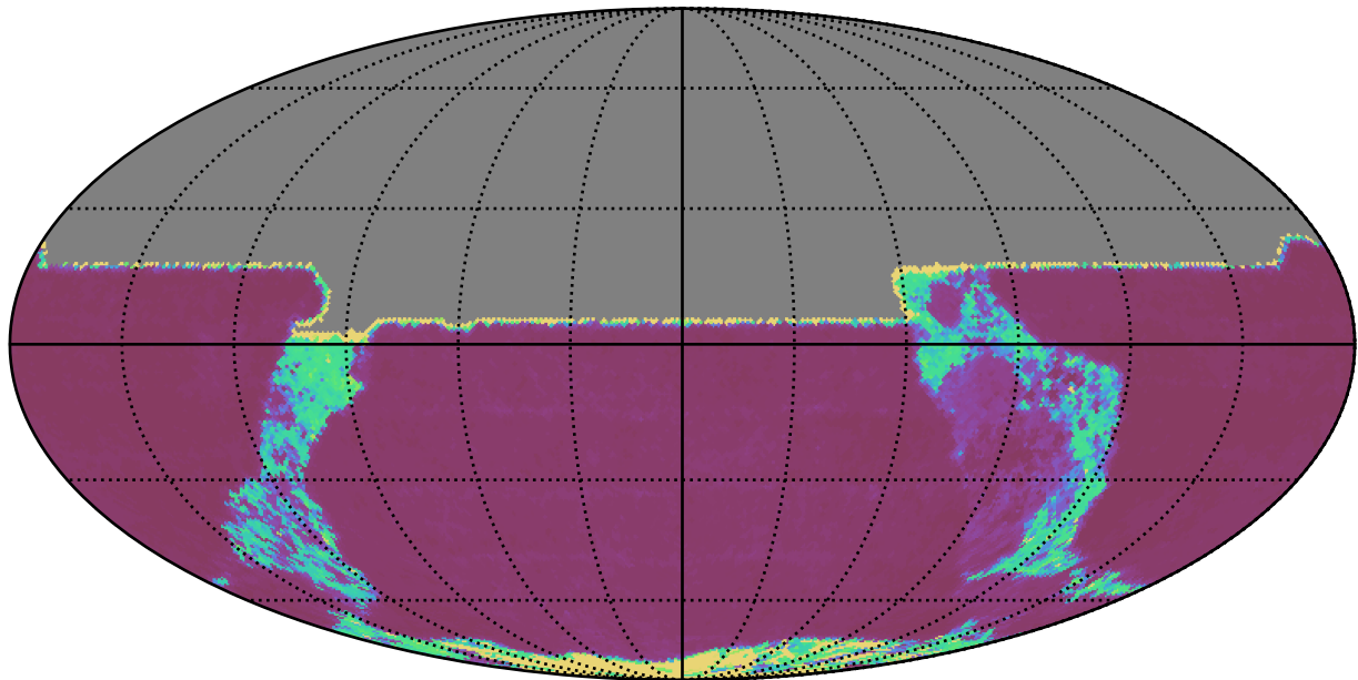
weather_cloudso18v3.4_10yrs All sky y band: 20thPercentile Inter-Night Gap
