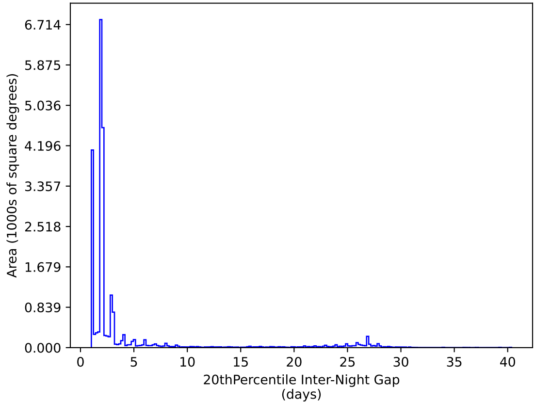
weather_cloudso18v3.4_10yrs All sky y band: 20thPercentile Inter-Night Gap
