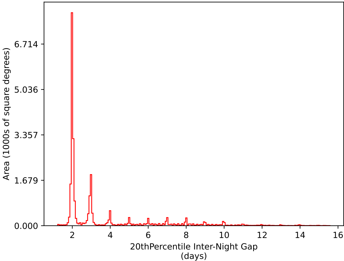
weather_cloudso18v3.4_10yrs All sky i band: 20thPercentile Inter-Night Gap
