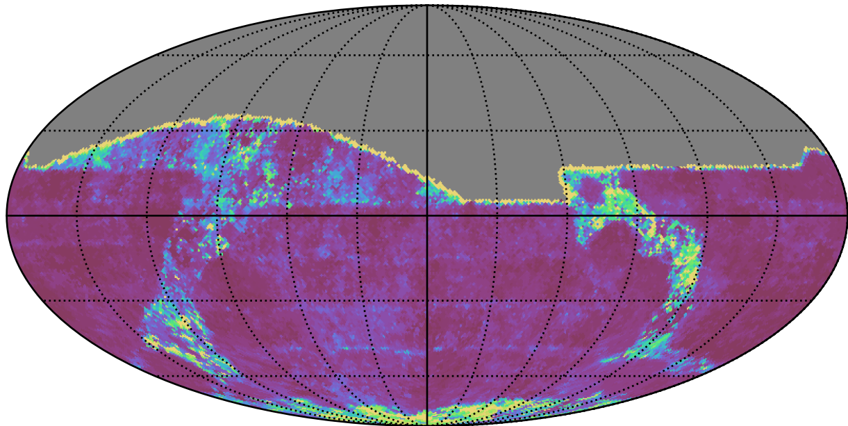
weather_cloudso18v3.4_10yrs All sky g band: 20thPercentile Inter-Night Gap
