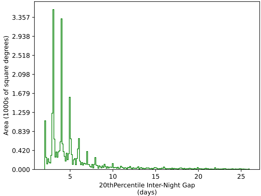
weather_cloudso18v3.4_10yrs All sky g band: 20thPercentile Inter-Night Gap
