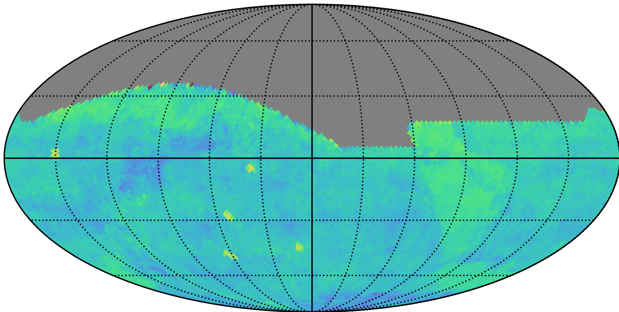
weather_cloudso18v3.4_10yrs (g or r or i): PairFraction
