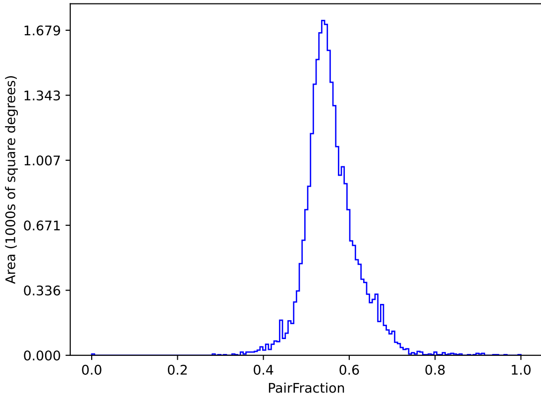
weather_cloudso18v3.4_10yrs (g or r or i): PairFraction
