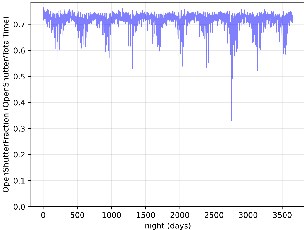
weather_cloudso18v3.4_10yrs : OpenShutterFraction
