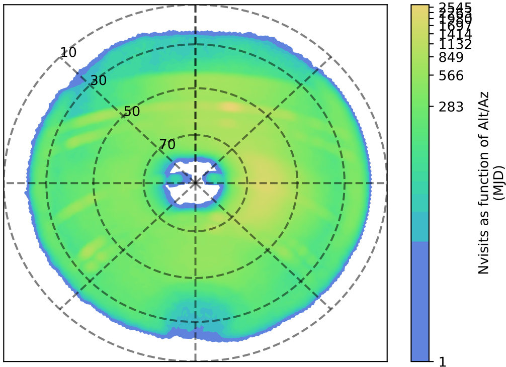
weather_cloudso18v3.4_10yrs z: Nvisits as function of Alt/Az
