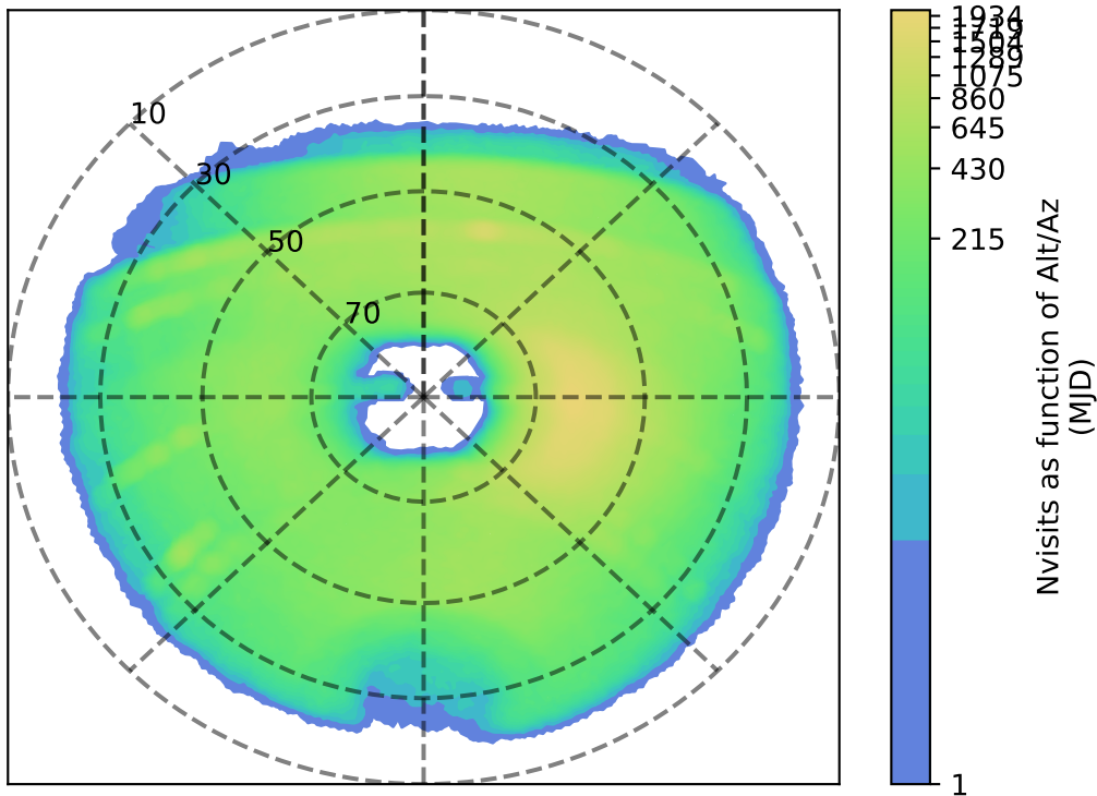
weather_cloudso18v3.4_10yrs y: Nvisits as function of Alt/Az
