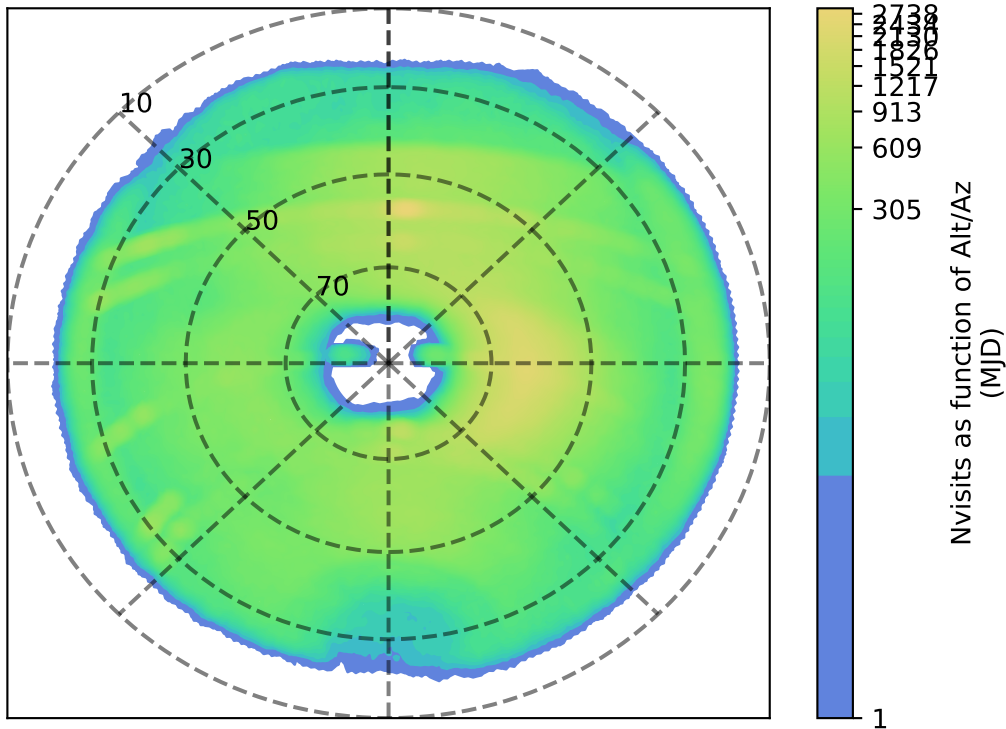
weather_cloudso18v3.4_10yrs i: Nvisits as function of Alt/Az
