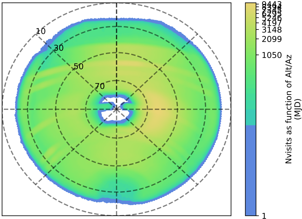
weather_cloudso18v3.4_10yrs : Nvisits as function of Alt/Az
