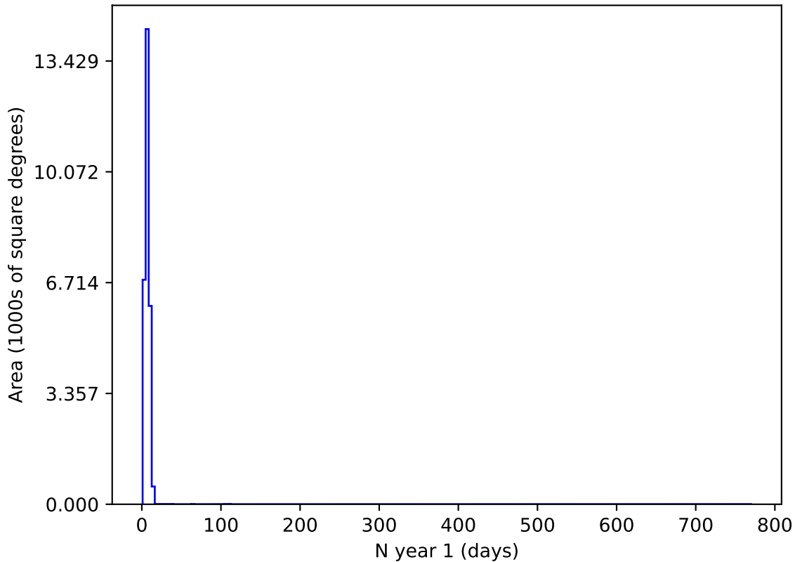
weather_cloudso18v3.4_10yrs g and night < 365: N year 1
