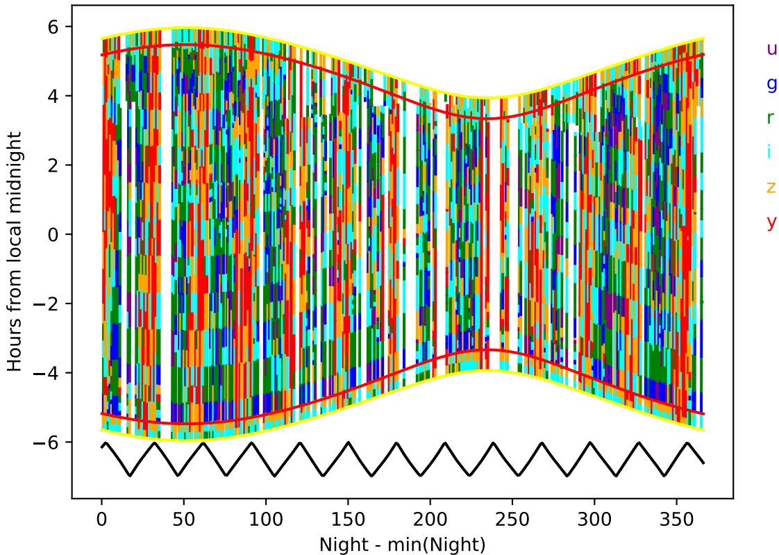
weather_cloudso18v3.4_10yrs year 9-10: Hourglass
