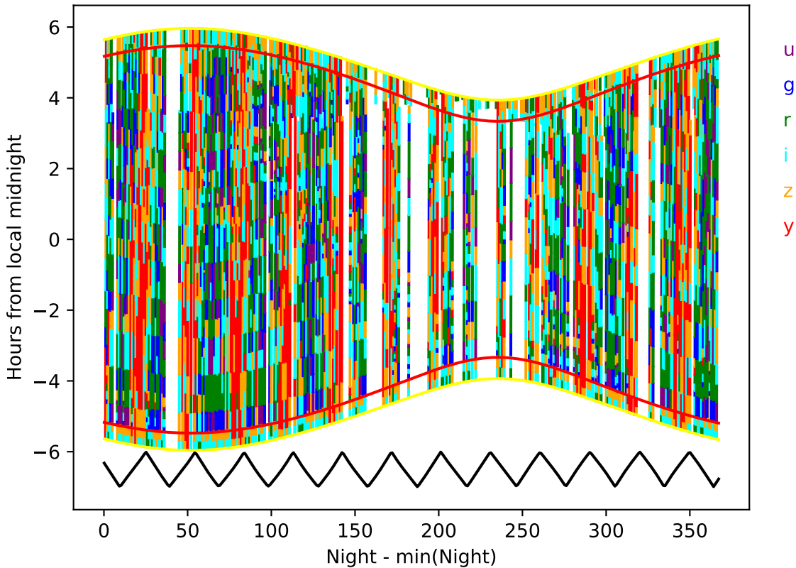
weather_cloudso18v3.4_10yrs year 7-8: Hourglass
