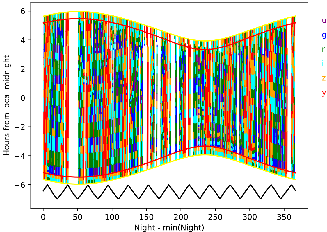
weather_cloudso18v3.4_10yrs year 6-7: Hourglass
