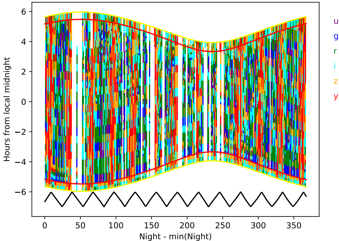
weather_cloudso18v3.4_10yrs year 3-4: Hourglass
