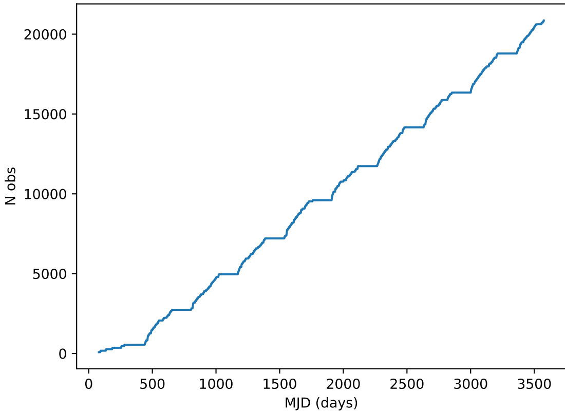
weather_cloudso18v3.4_10yrs note like DD:XMM_LSS%: Cumulative
