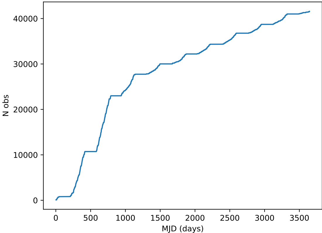
weather_cloudso18v3.4_10yrs note like DD:COSMOS%: Cumulative
