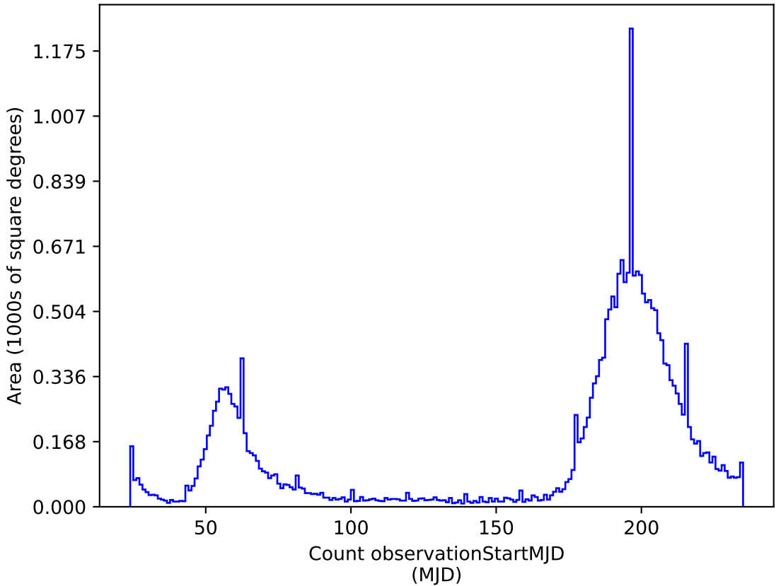
weather_cloudso18v3.4_10yrs r: Count observationStartMJD
