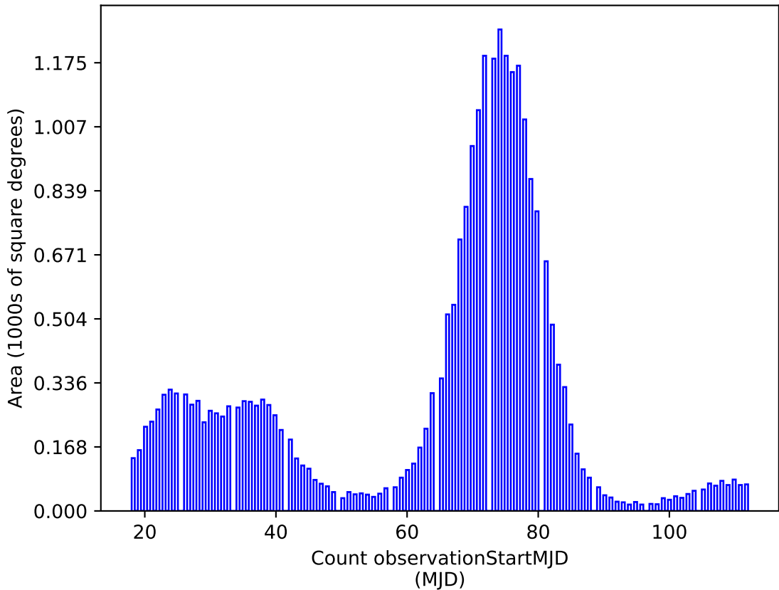
weather_cloudso18v3.4_10yrs g: Count observationStartMJD
