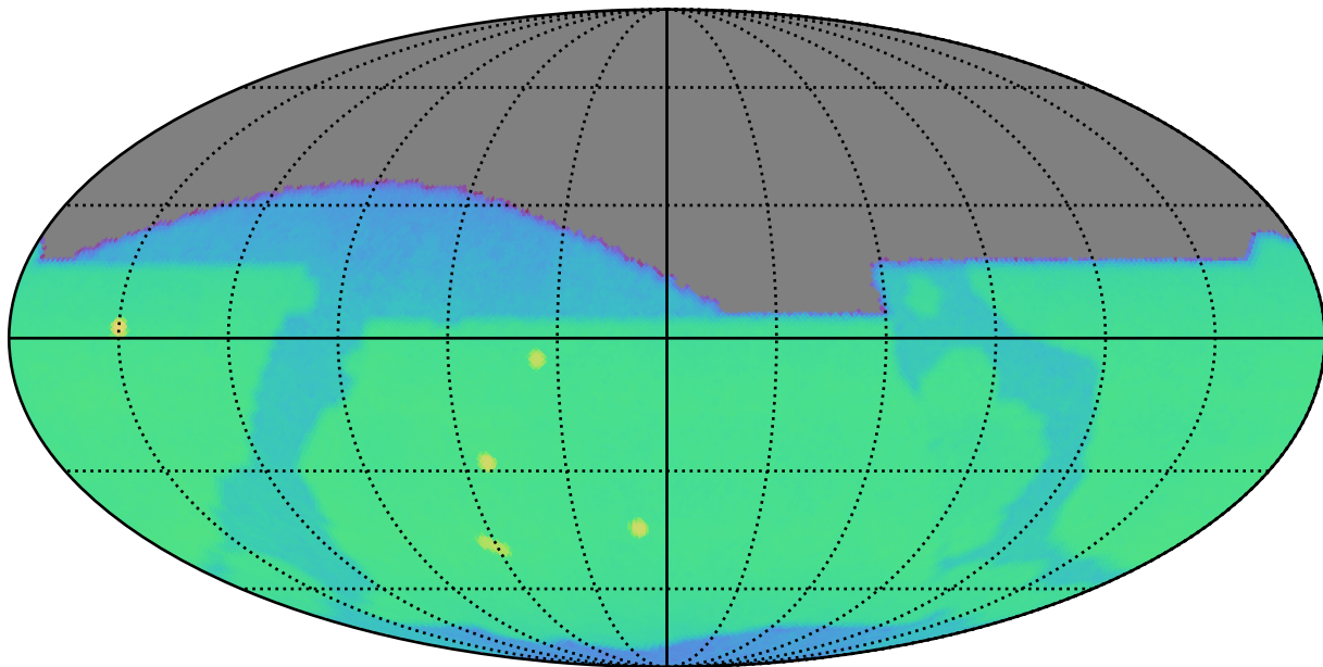
weather_cloudso18v3.4_10yrs z: CoaddM5
