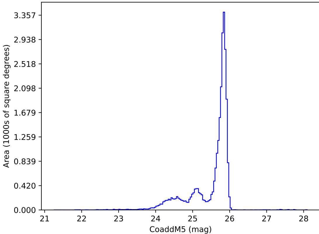
weather_cloudso18v3.4_10yrs z: CoaddM5
