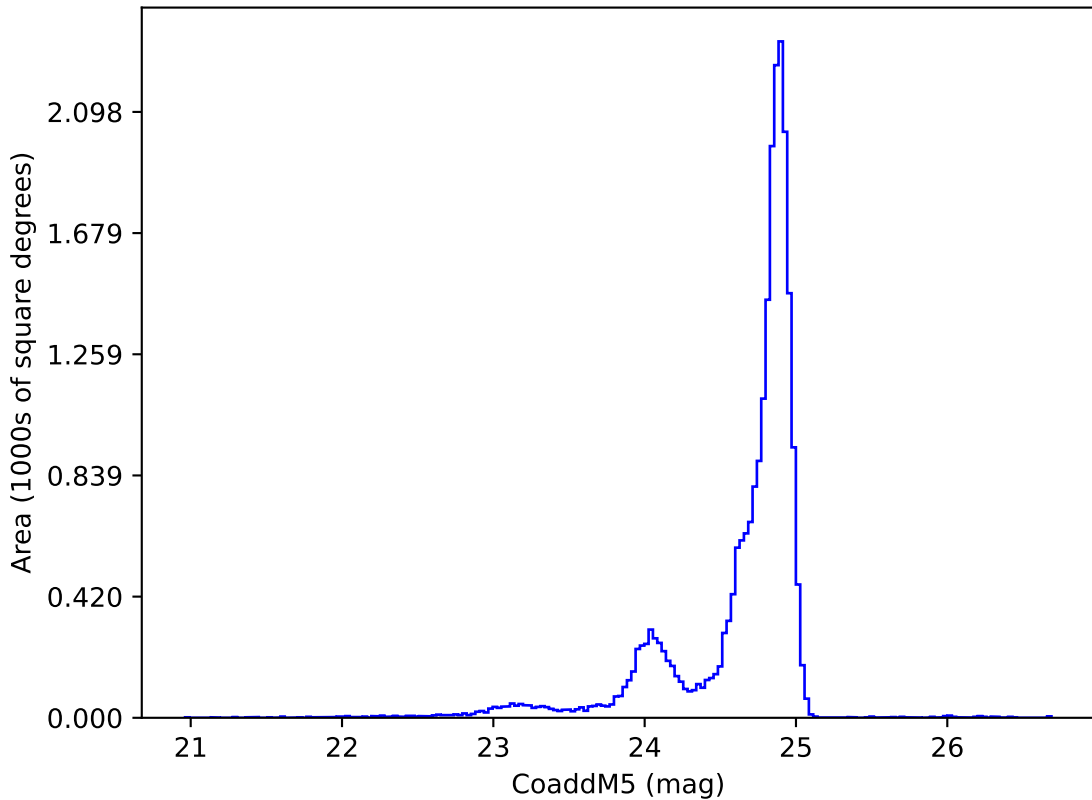
weather_cloudso18v3.4_10yrs y: CoaddM5
