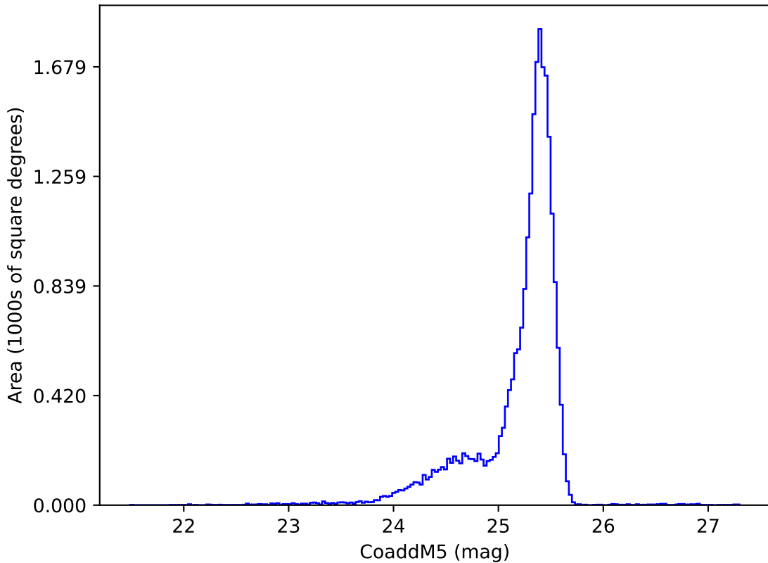
weather_cloudso18v3.4_10yrs u: CoaddM5
