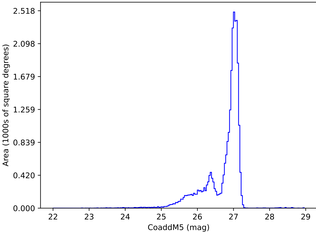
weather_cloudso18v3.4_10yrs r: CoaddM5
