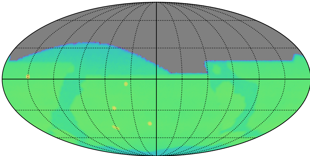
weather_cloudso18v3.4_10yrs : CoaddM5
