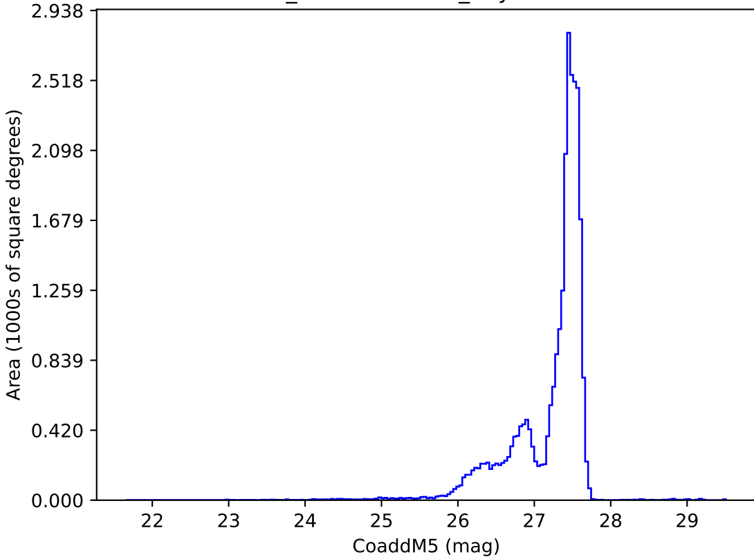
weather_cloudso18v3.4_10yrs : CoaddM5
