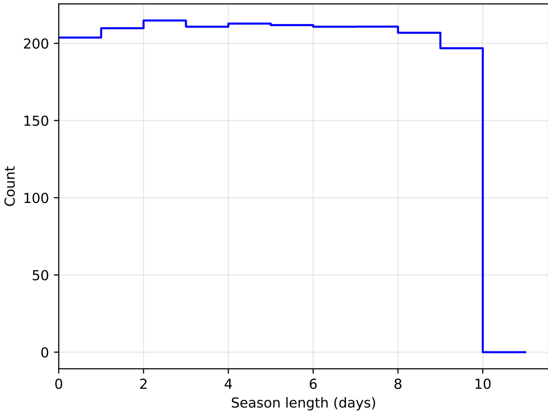
weather_cloudso18v3.4_10yrs DD:EDFS all bands: SeasonLength
