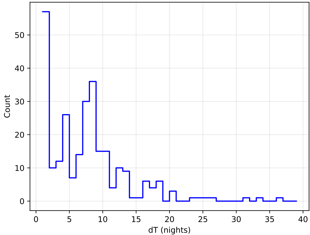
weather_cloudso18v3.4_10yrs all bands: DD:XMM_LSS Delta Nights Histogram
